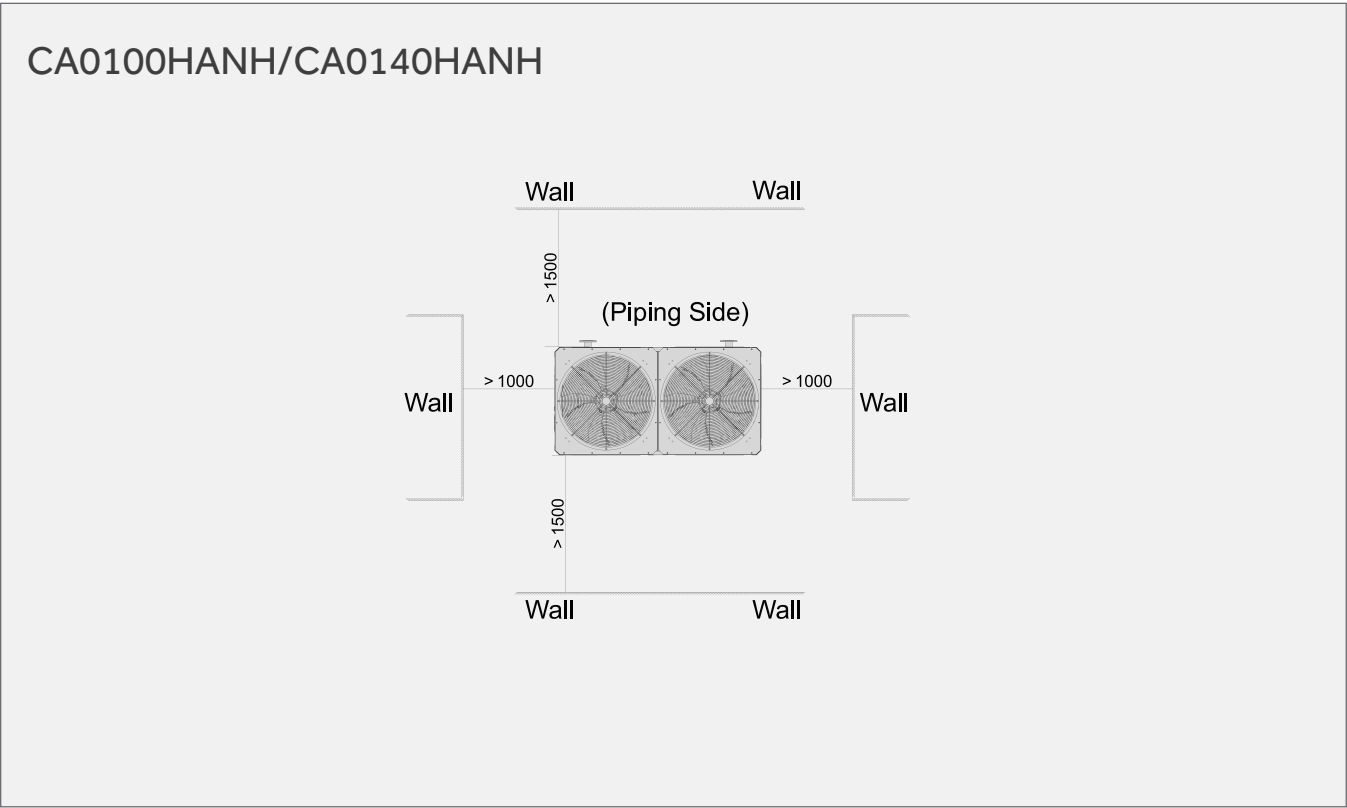
Installation Clearance (Single Chiller)
