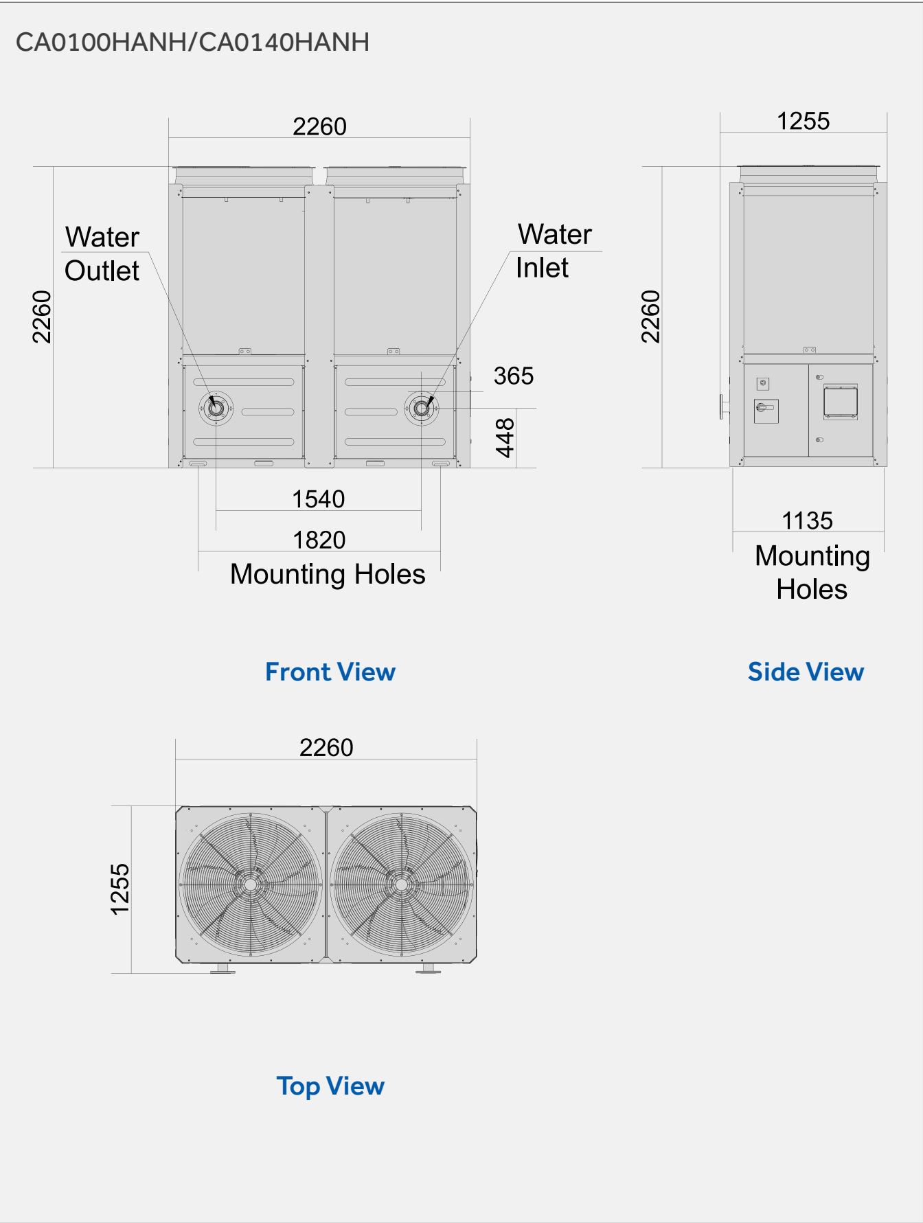
External Dimension
