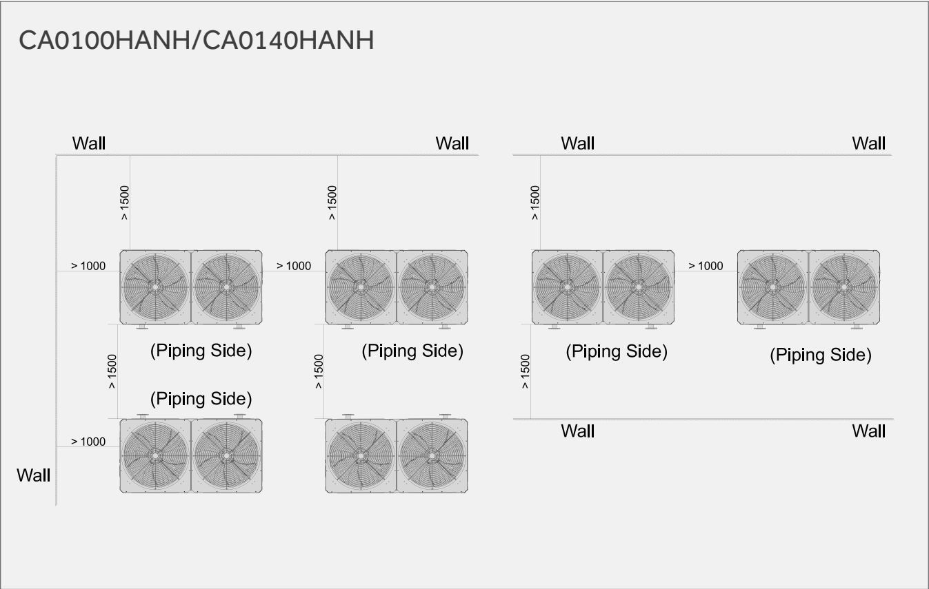
Installation Clearance (Multiple Chilers)
